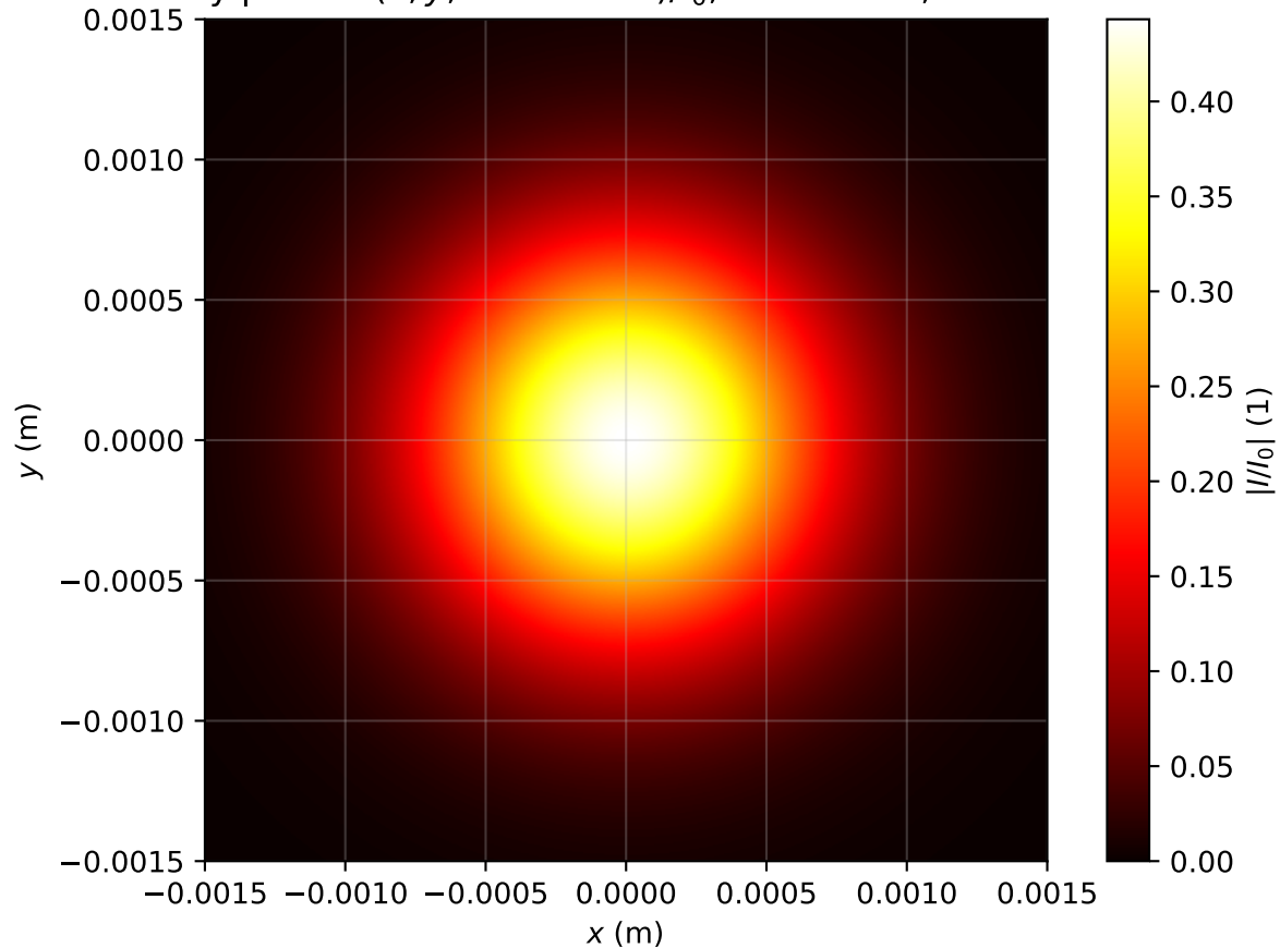
Intensity profile I(x, y, z = 2.627m)/I_0 , P_{in}=0.2P_{cr} , artificial time
